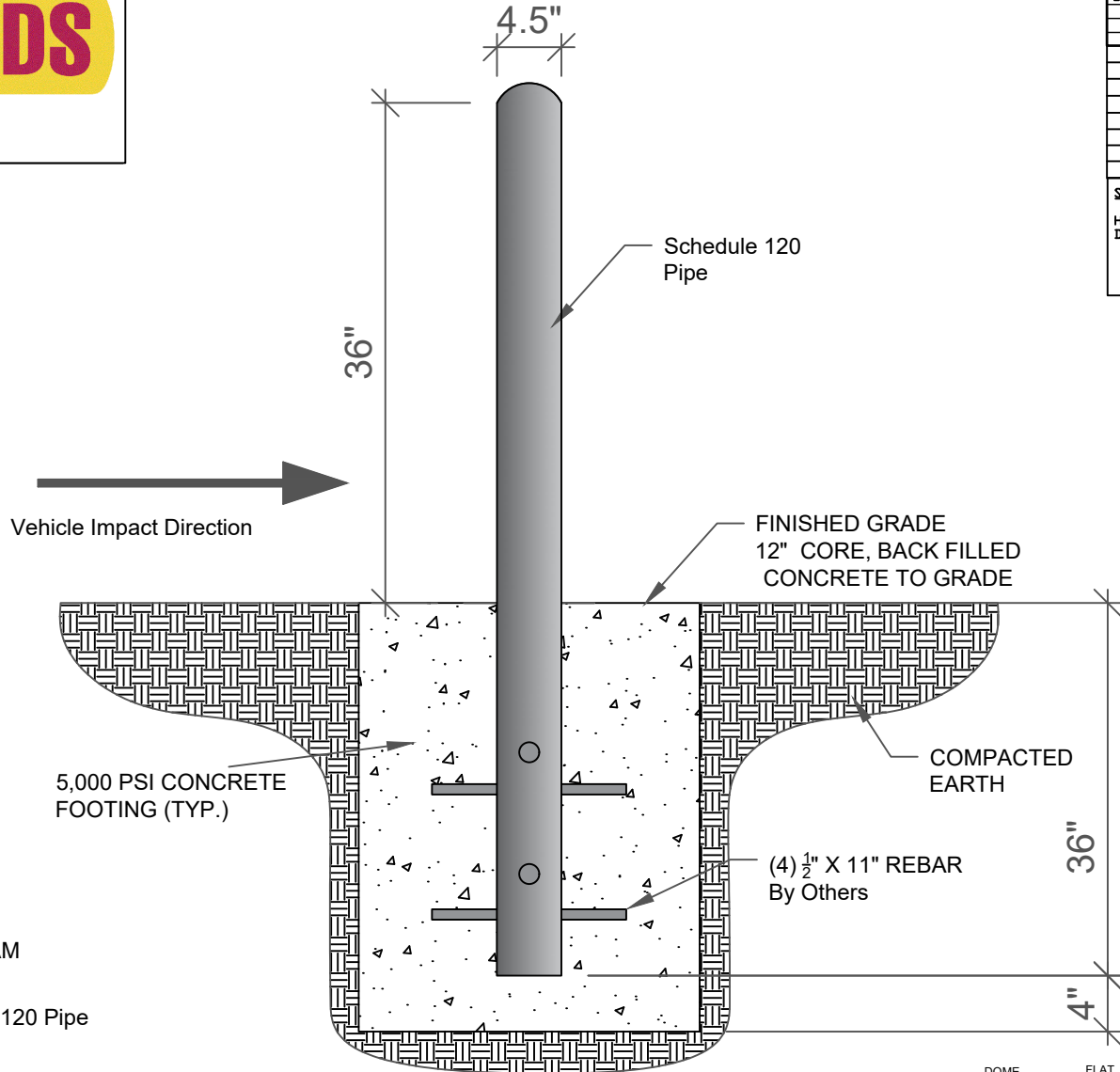
END VIEW-FOUNDATION
