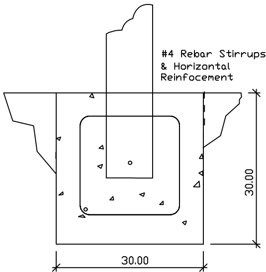
END VIEW - FOUNDATION
