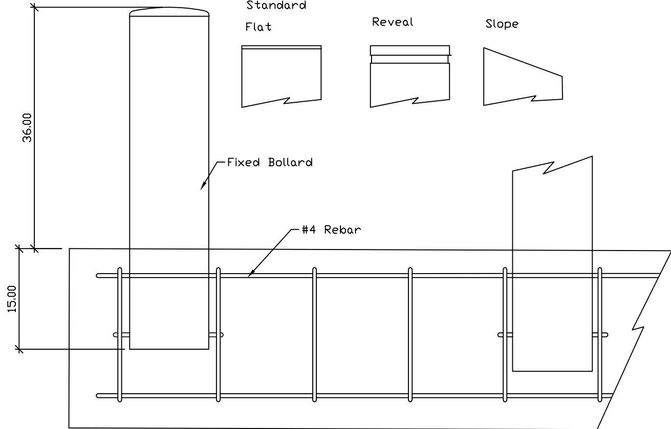
ELEVATION VIEW - FOUNDATION (CONCEPTUAL DESIGN ONLY)
