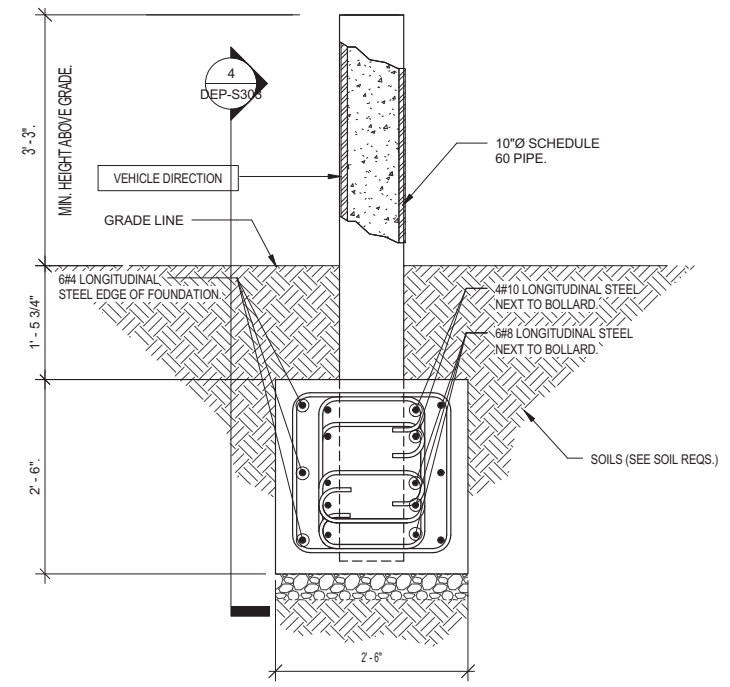
5 K-4 ANTI - RAM BOLLARD (SECTION) 3/4" = 1'-0"
