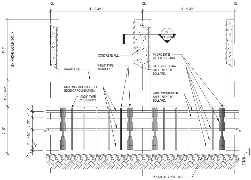
4 K-4 ANTI - RAM BOLLARD 3/4" = 1'-0"
